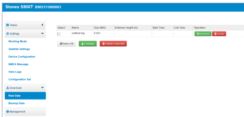
Figure 2.3.1 download page
