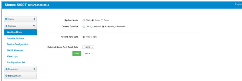
Figure 2.2.1 setting page
